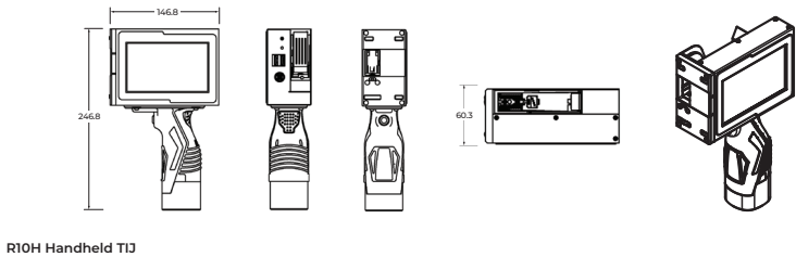
R10H Handheld TIJ
